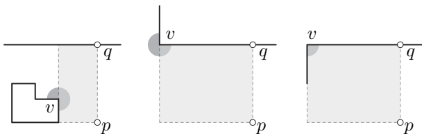
Figure 8: Illustration of the proof of Theorem 5.
