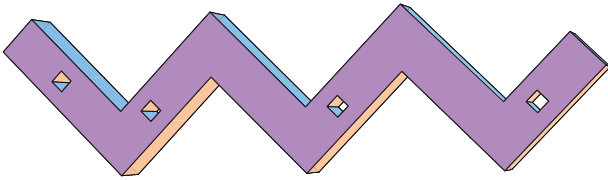
Figure 4: A polyhedron that achieves the tight left-hand side bound in Theorem 2.
